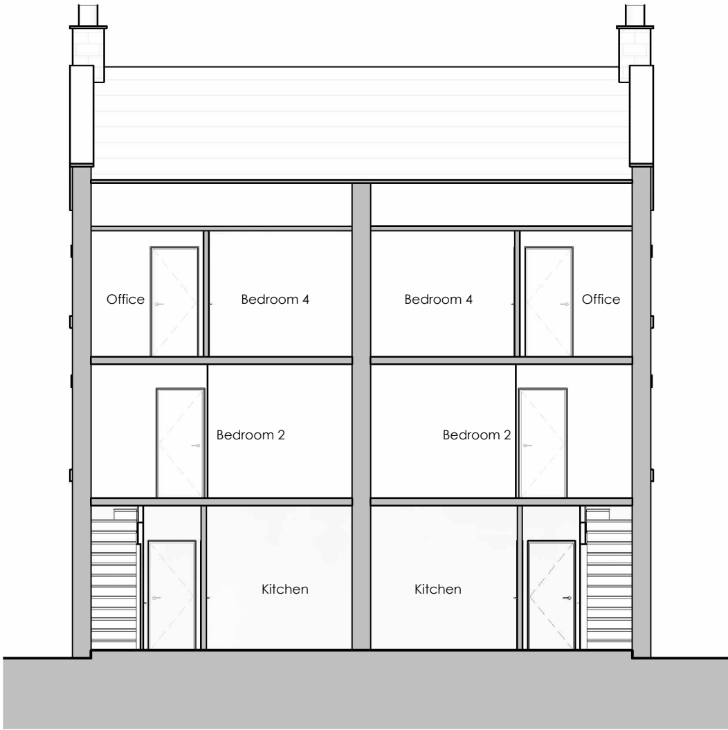
Proposed Section AA 1 : 100
